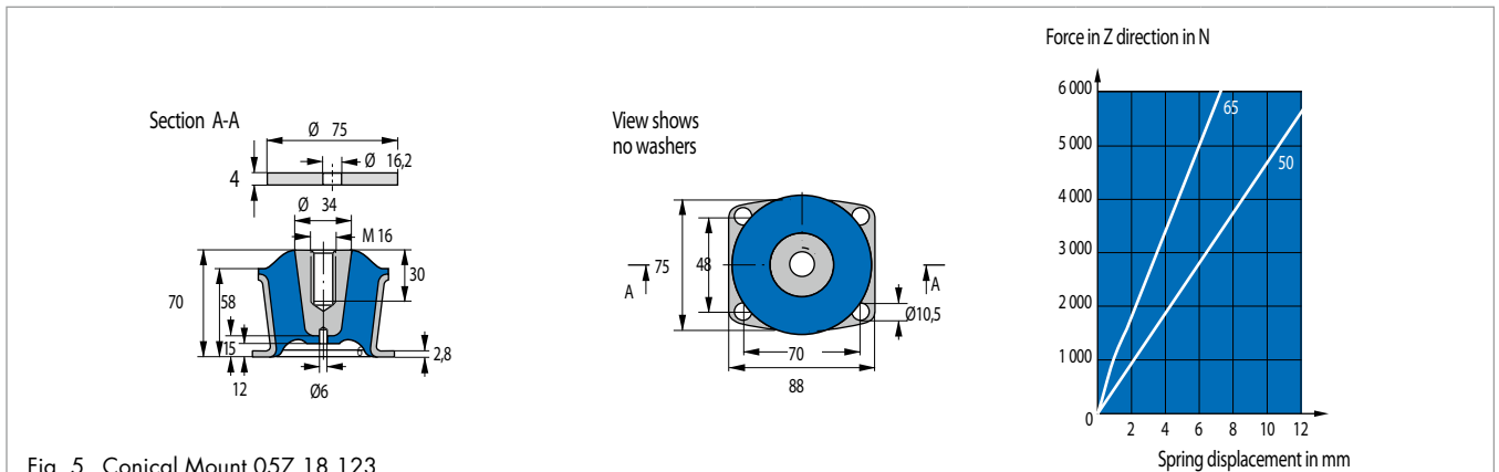
Fig. 5 Conical Mount 057 18 123
