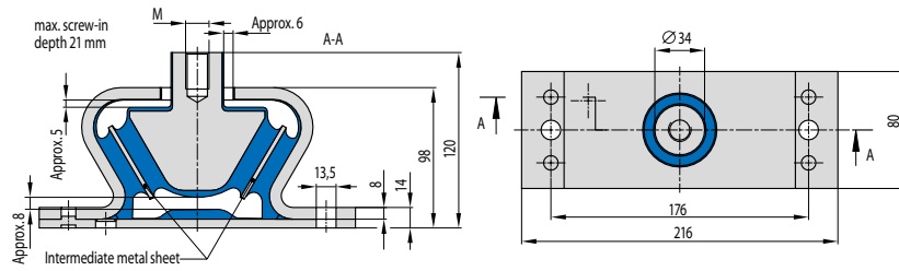
Fig. 3 Tapered Mounts 033 18 720, 033 18 730
