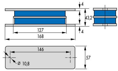
Fig. 5 Flat Mount 051 18 002
