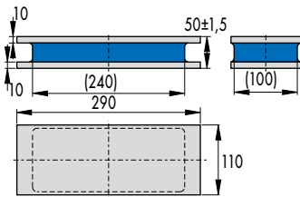
Fig. 6 Flat Mount 051 18 719
