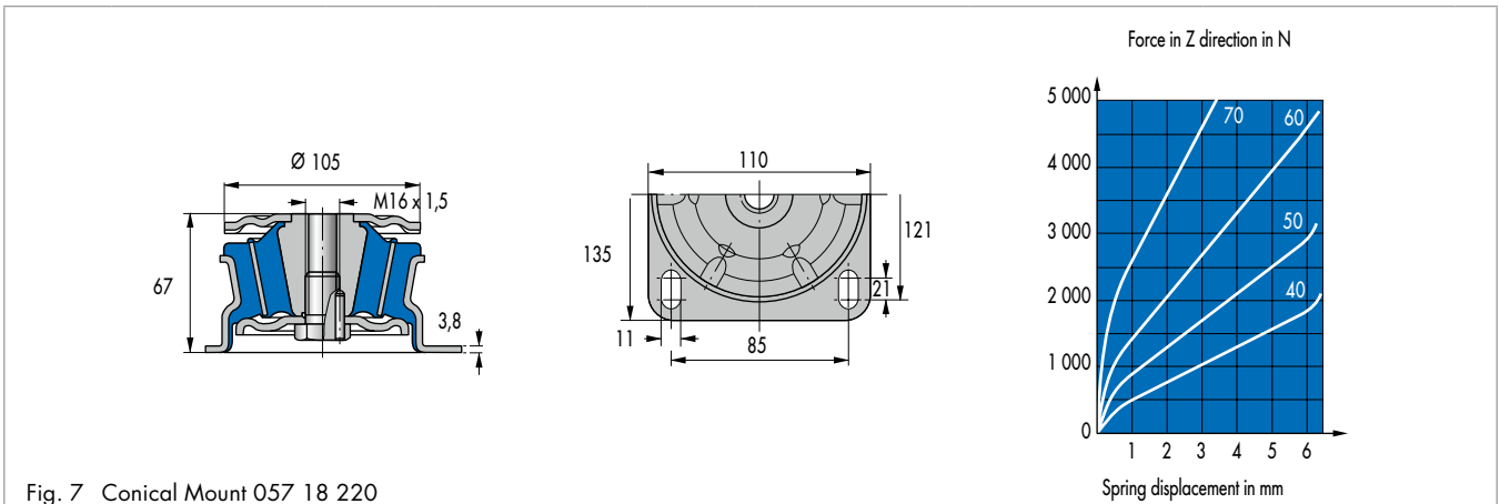
Fig. 7 Conical Mount 057 18 220
