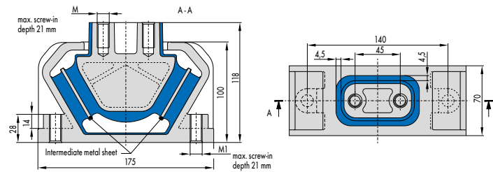
Fig. 4 Tapered Mounts 033 18 700, 033 18 701
