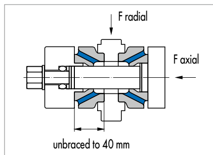
Fig. 2 Fitting & installation instructions: Top Mount with load directions
