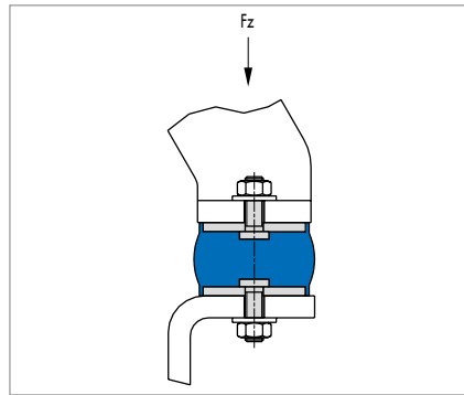
Fig. 4 Compressive loading
