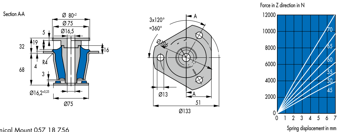
Fig. 15 Conical Mount 057 18 756
