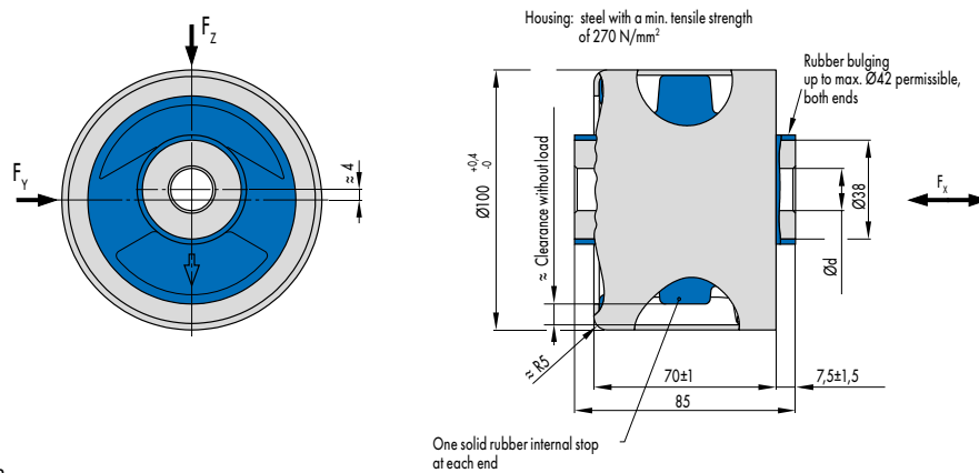
Fig. 4 Hydro Bush
