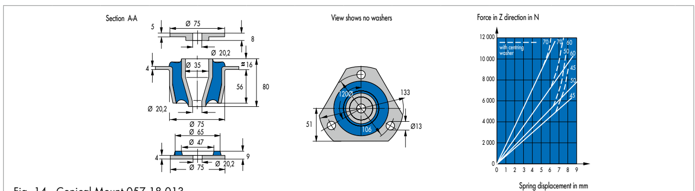
Fig. 14 Conical Mount 057 18 013
