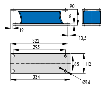
Fig. 8 Flat Mount 051 18 723
