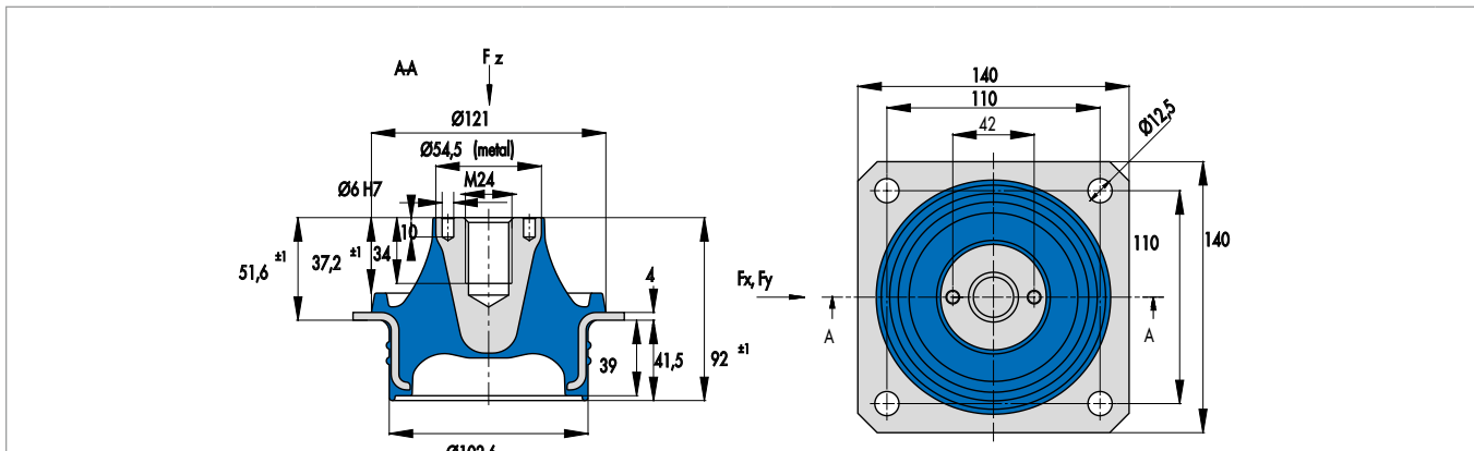
Fig. 20 Conical Mount 057 18 795
