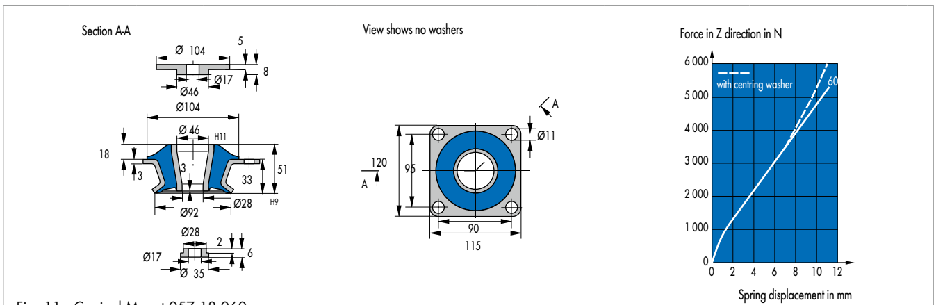
Fig. 11 Conical Mount 057 18 060
