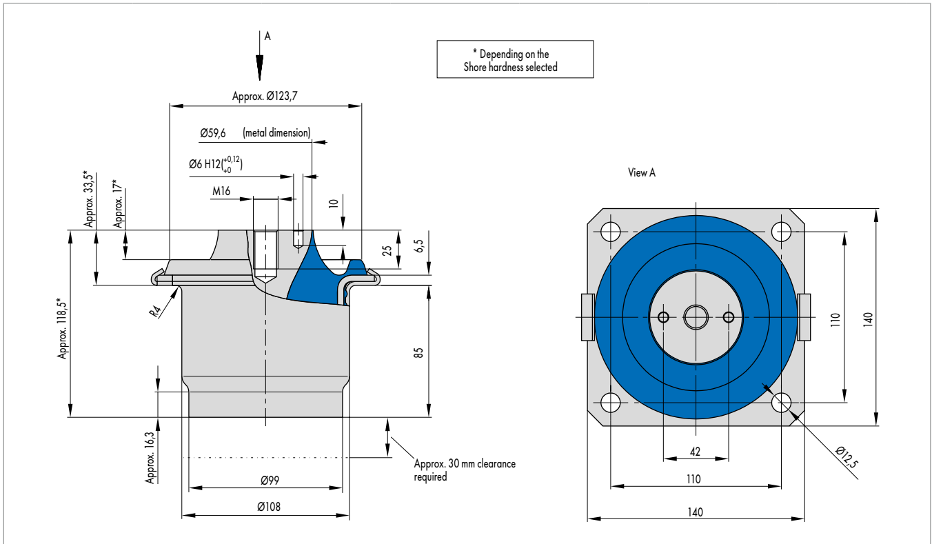
Fig. 6 Hydro Mount VL 036 18 704
