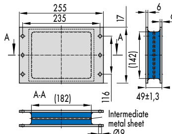
Fig. 7 Flat Mount 051 18 720
