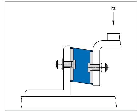
Fig. 5 Shear loading
