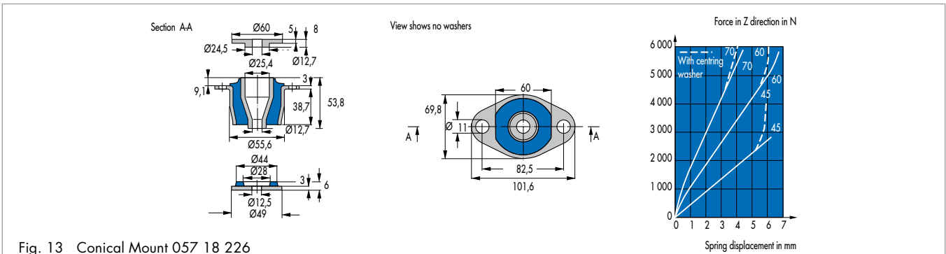
Fig. 13 Conical Mount 057 18 226
